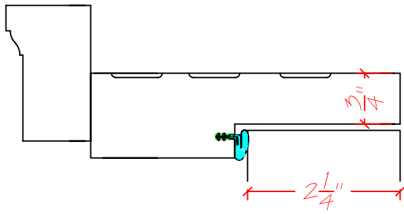
Jamb leg - plan view
