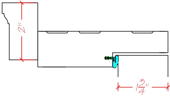
Jamb head - cross section
