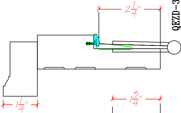
Jamb leg - plan view
